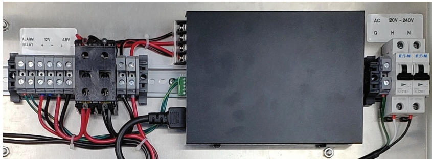
ICT24048-7BC2 IntelliCharge 48 volt, 7.5 Amp DC power supply and charger shown on DIN rail
